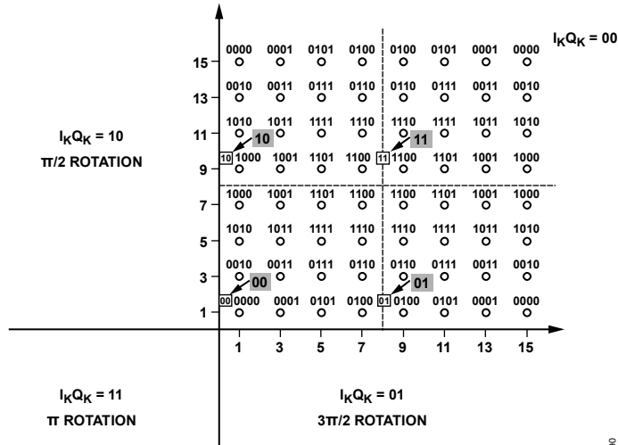
Figure 125. DVB 256-QAM Constellation
